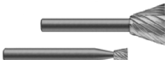
H.S.S. Midget-Mill® Single Cut Chip Breakers
